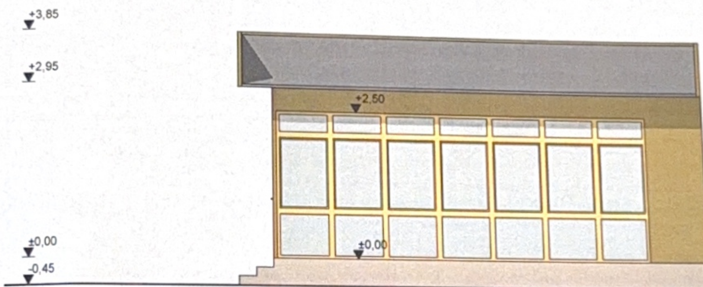
FATADA VEST
