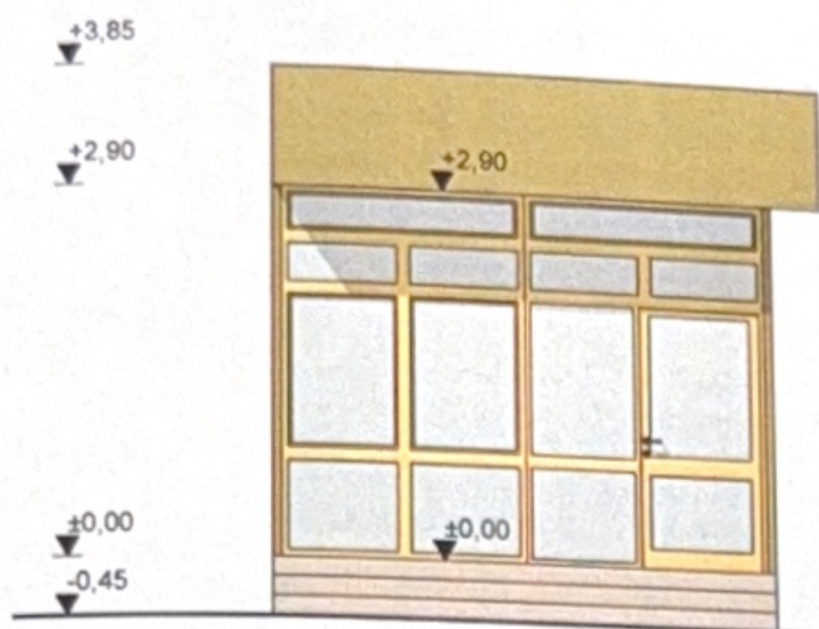
FATADA VEST
